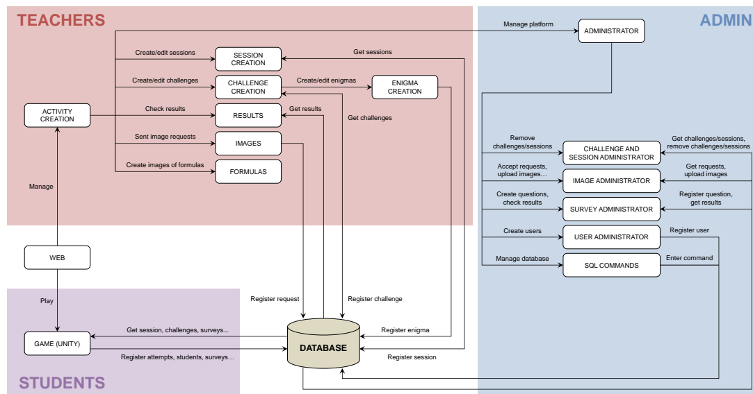
Figure 8: The main modules and functionalities of the TAECon platform.
