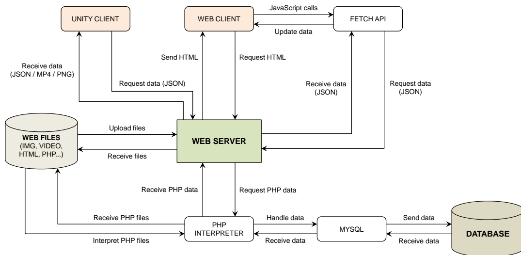
Figure 7: Client-server architecture of the TAECon platform.
